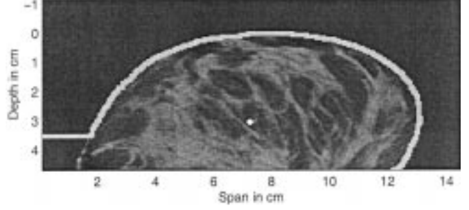
Fig. 2. Two-dimensional dielectric-properties breast model derived from an MRI scan. A 2-mm-diameter malignant tumor has been inserted at a depth of 3.1 cm.
